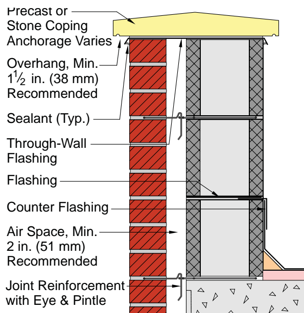
Figure 18 Metal Coping on Cavity Wall Parapet
