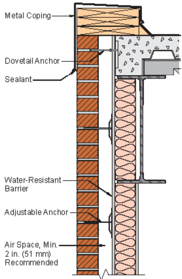
Figure 19 Non-Parapet Wall
