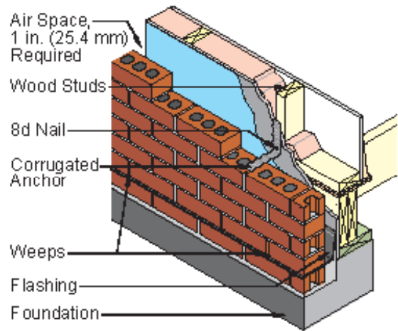
Figure 2 Brick Veneer/Wood Stud Wall
