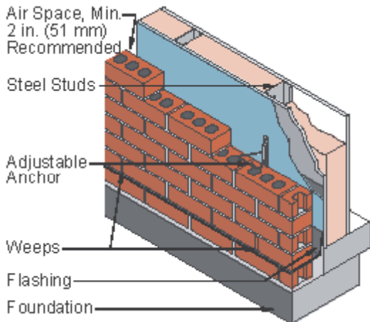
Figure 3 Brick Veneer/Steel Stud Wall
