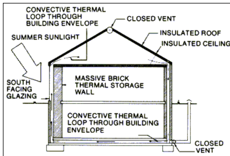
Cavity Wall System Heating Mode
