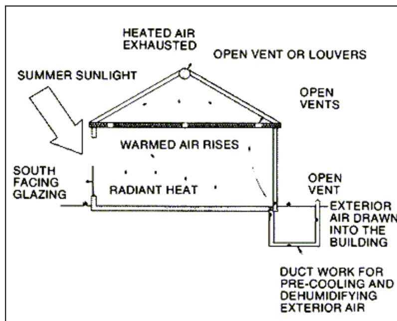
Pre-Cooling and Dehumidification of Exterior Air
