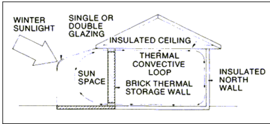
Attached Sunspace
