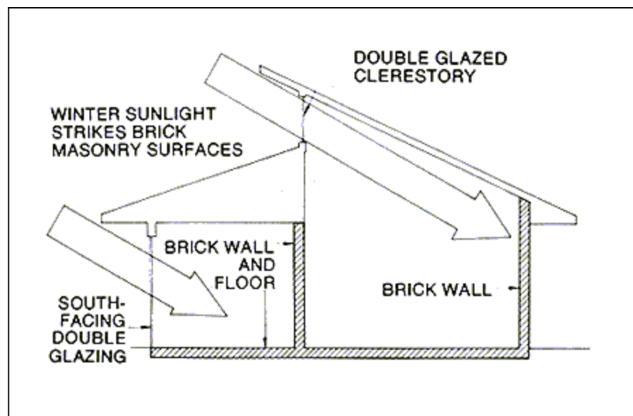
Increased Building Depth Using Direct Gain System with Clerestory
