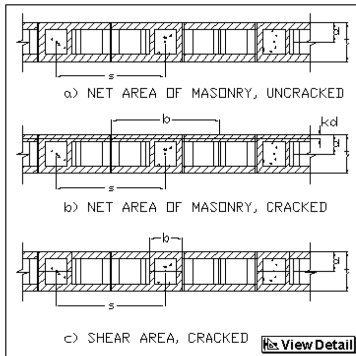
Effective Areas for Partially Grouted, Hollow Unit Masonry Walls
