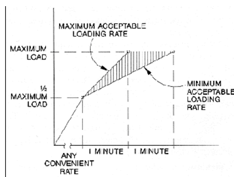
Compressive Test Loading Rate FIG. 2
