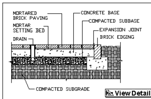
Mortared Brick Paving
