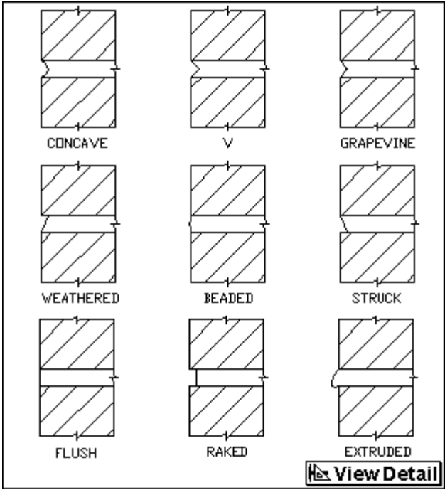
Typical Mortar Joints
