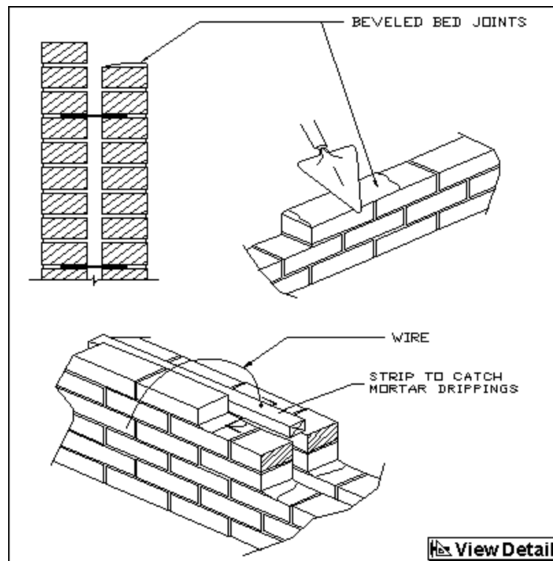
Keeping the Cavity Clean
