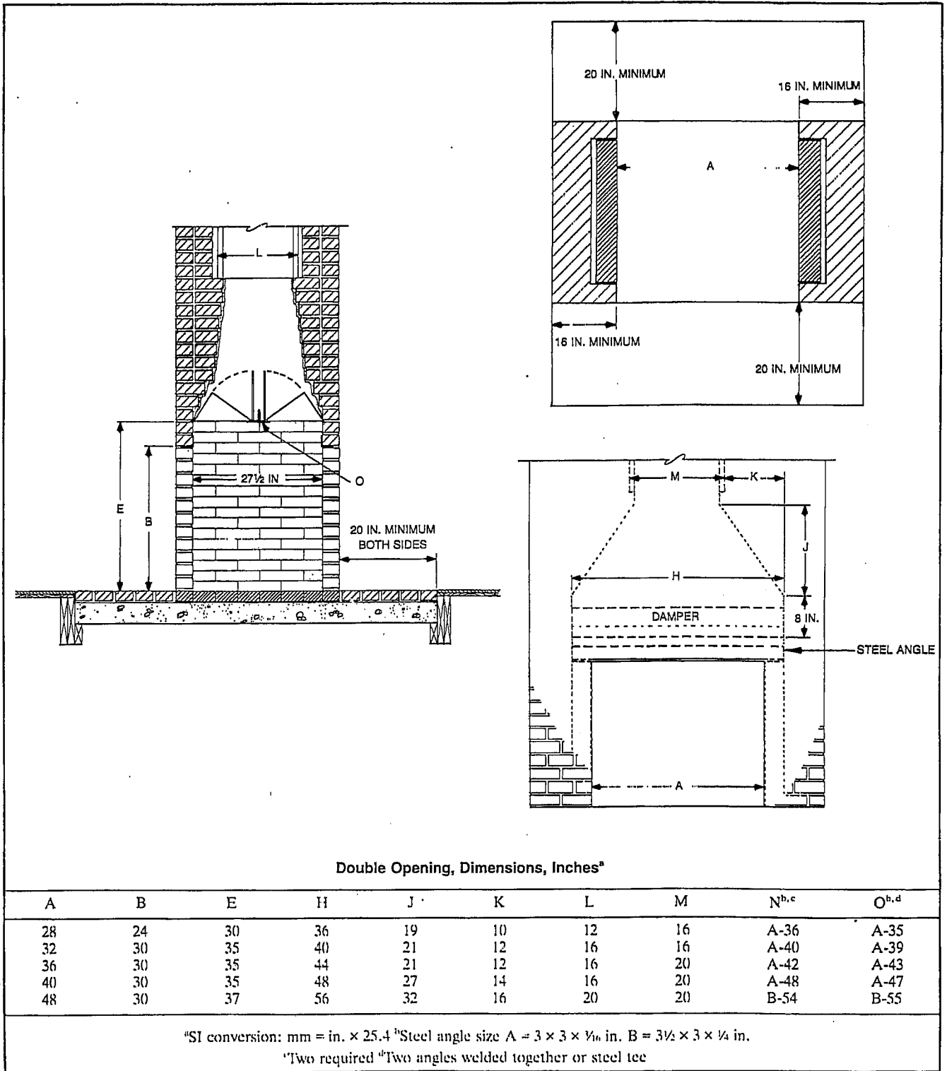
Two-Face Fireplace
