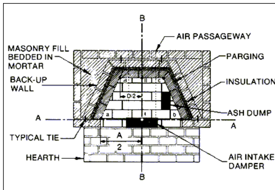
Combustion Chamber Plan
