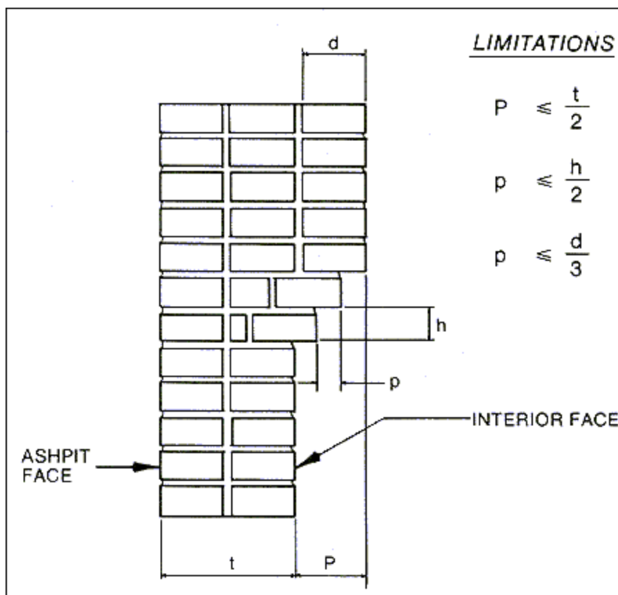
Corbeling Limitations
