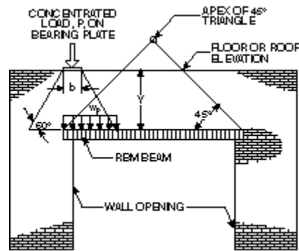
Loads on RBM Beam FIG. 4
